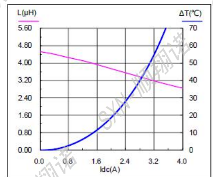
SMMS0420-4R7M
