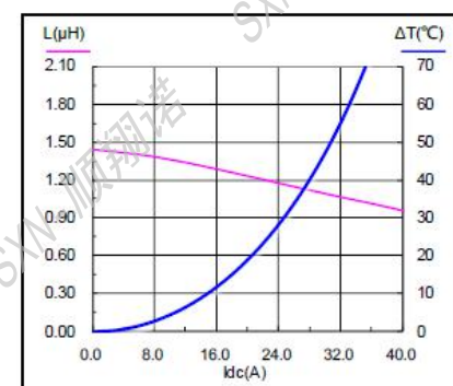
SMMS1350-1R5M
