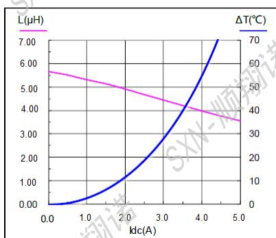
SMMS0520-5R6M
